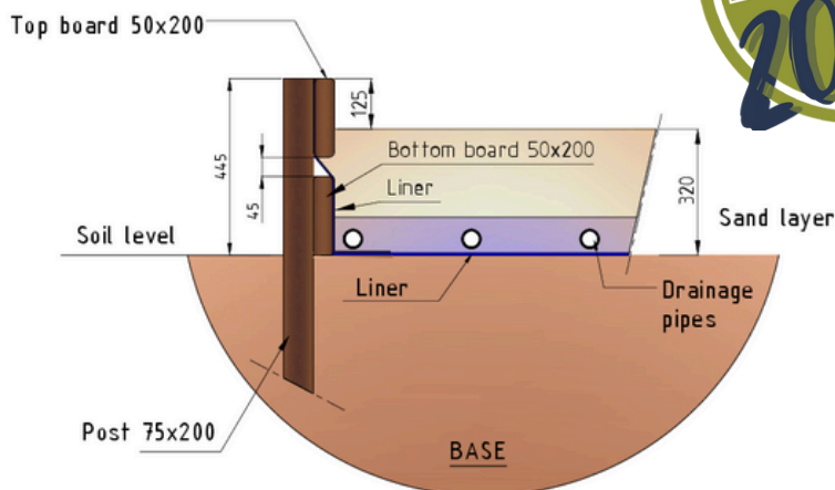
TYPICAL CROSS-SECTION - TIMBER SURROUND
